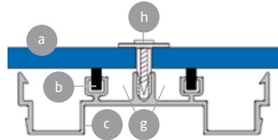
Horizontal section
